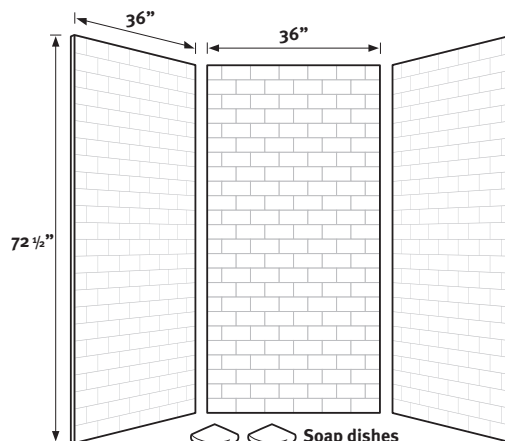
Model STMK 72-3636
