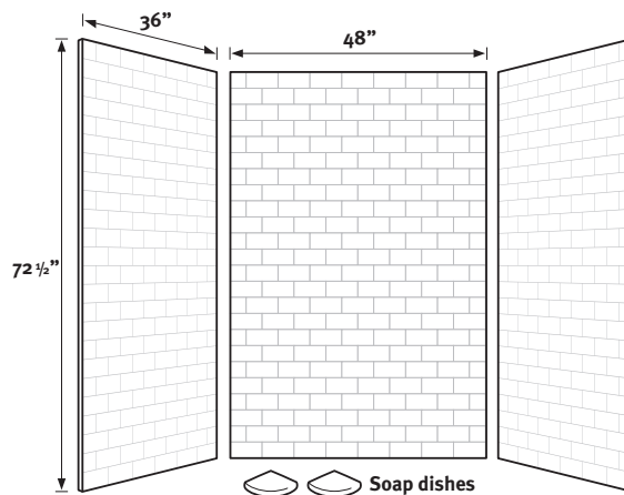
Model STMK72-3648
